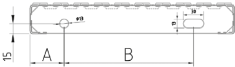
LASCHE FORMSTEP N
